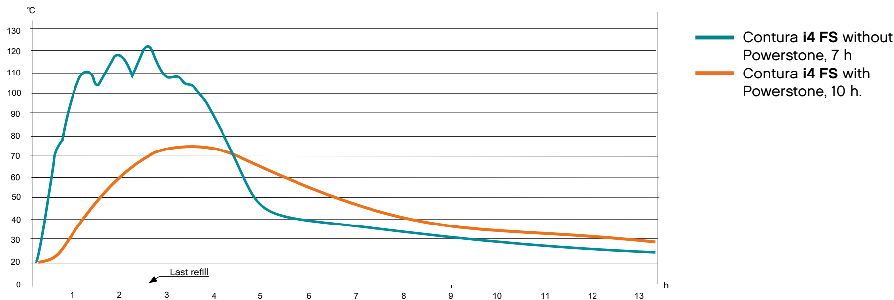
Temperature curve Contura i4 FS
